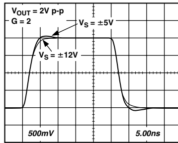
TPC 83. AD8130 Transient Response vs. Supply, V_{OUT} = 2\ V\ p-p , G = 2
