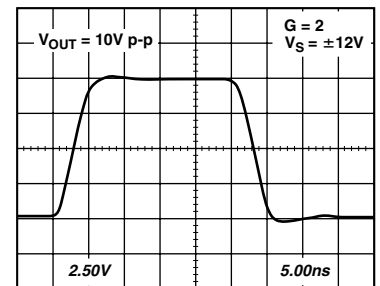
TPC 87. AD8130 Transient Response, V_{OUT} = 10\ V\ p-p , G = 2 , V_S = \pm 12\ V
