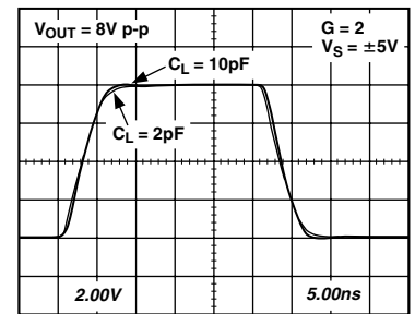
TPC 84. AD8130 Transient Response vs. Load Capacitance, V_{OUT} = 8\ V\ p-p
