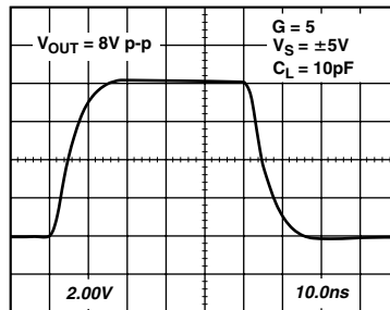
TPC 89. AD8130 Transient Response, V_{OUT} = 8\ V\ p-p , G = 5 , V_S = \pm 5\ V
