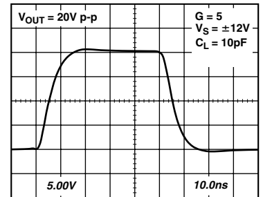
TPC 90. AD8130 Transient Response, V_{OUT} = 20\ V\ p-p , G = 5 , V_S = \pm 12\ V
