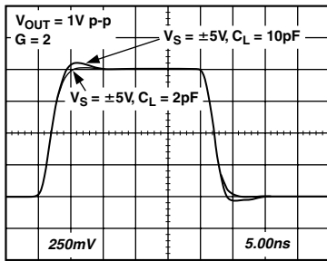
TPC 82. AD8130 Transient Response vs. Load Capacitance, V_{OUT} = 1\ V\ p-p , G = 2
